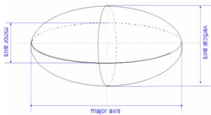
Figure 17.2: 3D-Ellipsoid and its axes
