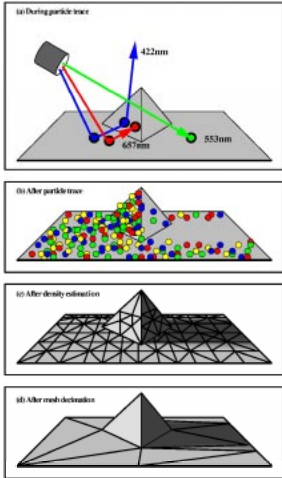
Figure 11: (a) and (b) Particle Tracing: Power-carrying particles, each with a specific wavelength, are emitted from each luminaire using an appropriate spectral radiant intensity distribution and tracked as they travel through the environment until they are absorbed. Each time a particle hits a surface it is probabilistically absorbed or scattered in a new direction according to the BRDF of the surface. A list of all particle “hit points” is generated and saved. (c) Density Estimation: The stored hit points are used to construct approximate lighting functions on each surface. The illumination on a surface is proportional to the density of the hit points. To reconstruct luminous and chromatic exitance, the hits are weighted by the surface reflectance and the CIE XYZ response functions and local linear density estimation is applied. The result is a Gouraud-shaded mesh of triangles with three color channels suitable for direct display. (d) Mesh Decimation: The initial mesh is generated conservatively and can be decimated by progressively removing vertices as long as the resulting change is below a perceptually-based threshold. Although not part of the simulation/measurement paradigm, it is useful to have the capability to rapidly display the rendered scene.
