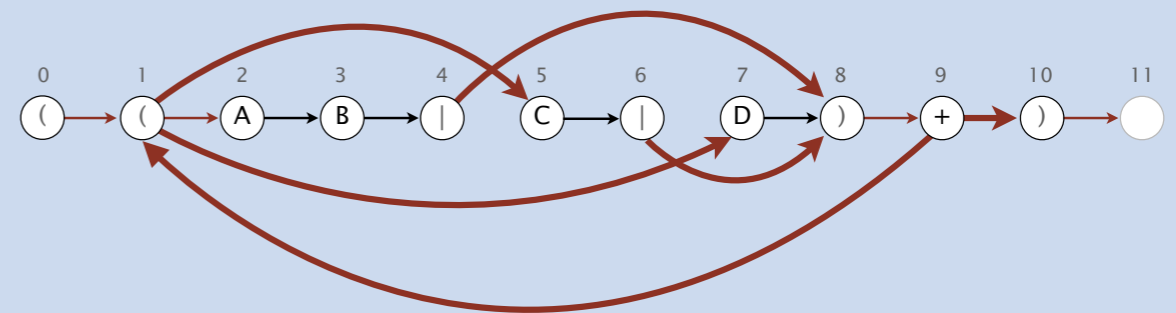
NFA corresponding to the pattern ( ( A B | C | D ) + )
