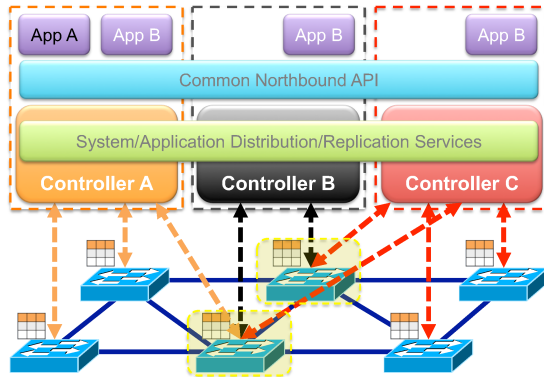
Figure 2: Secure & Dependable SDN
