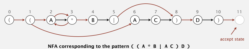
NFA corresponding to the pattern ((A * B | A C) D)
