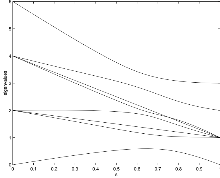
Figure 6: The eight levels of \tilde{H}(s) for the 3-bit problem with H_{\mathbb{P}} and H_{\mathbb{B}} given by (3.5).
