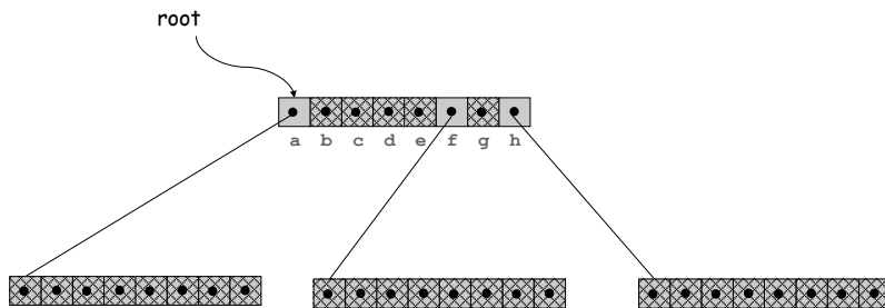
8-way trie
