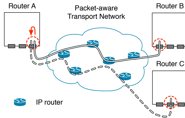
(b) Packet-aware transport network
