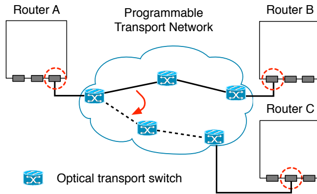
(a) Programmable transport network
