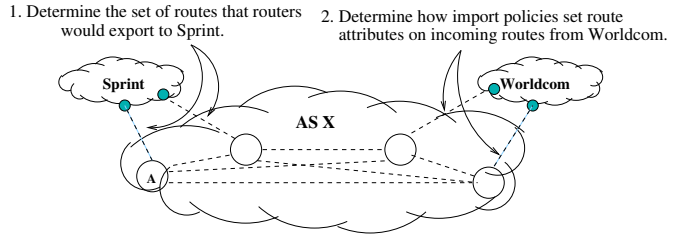
Figure 6. How rcc computes route propagation.
