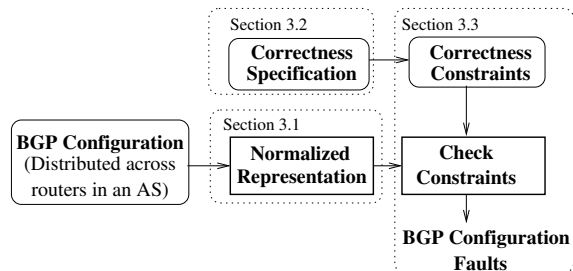
Figure 2. Overview of rcc .
