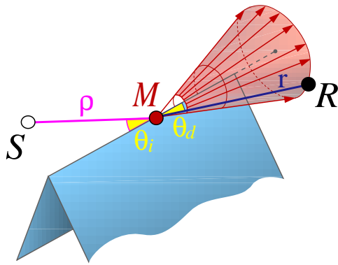
Figure 11: Rays diffracted by a 3D wedge according to the Uniform Theory of Diffraction. The angle \theta_d of the cone is equal to the angle \theta_i between the incident ray and the edge.
