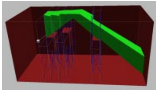
Figure 13: A beam clipped and reflected at cell boundaries.
