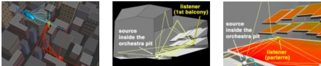
Figure 27: Visualizations of sound paths in different environments. Diffraction of sound in a city environment is shown on the left, while early propagation paths for a source located in the orchestra pit of an opera house are shown in the middle and right images. Note the diffracted paths over the lip of the pit and balconies (cyan arrows).
