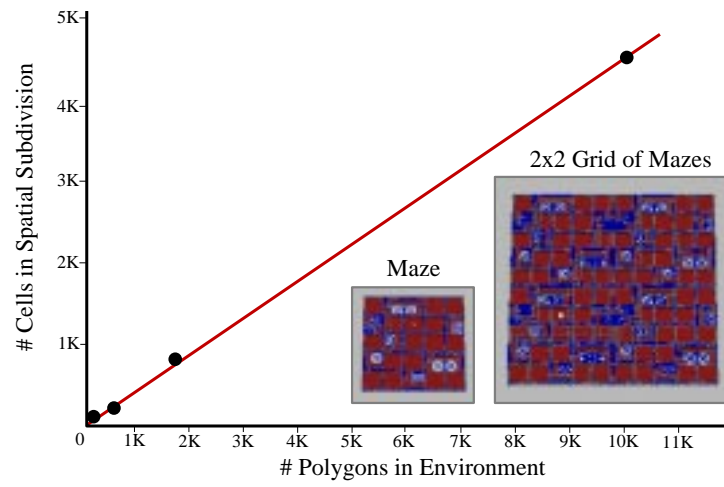
Figure 19: Plot of subdivision size vs. polygonal complexity.
