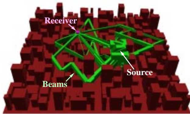
Figure 25: Beams (green) containing all eighth-order specular reflection paths from a source to a receiver in City model.
