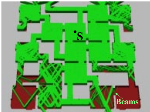
Figure 24: Eighth-order specular reflection beams (left) and predicted power levels (right) in Maze model.
