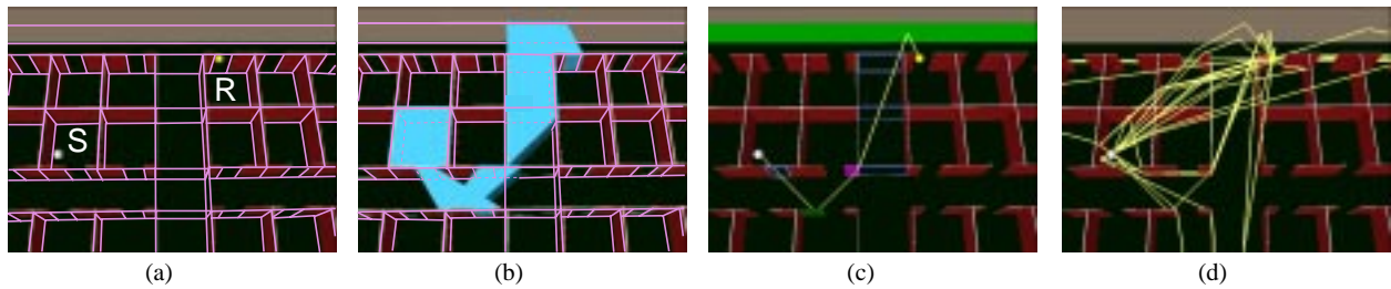
Figure 7: Results of each phase of execution: (a) Virtual environment (office cubicles) with source S , receiver R , and spatial subdivision marked in pink, (b) Example reflected and diffracted beam (cyan) containing the receiver, (c) Path generated for the corresponding sequence of opaque faces (green), transparent faces (purple), and edges (magenta), and (d) Many paths found for different sequences from S to R .
