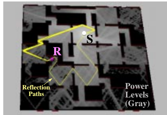
Figure 24: Eighth-order specular reflection beams (left) and predicted power levels (right) in Maze model.
