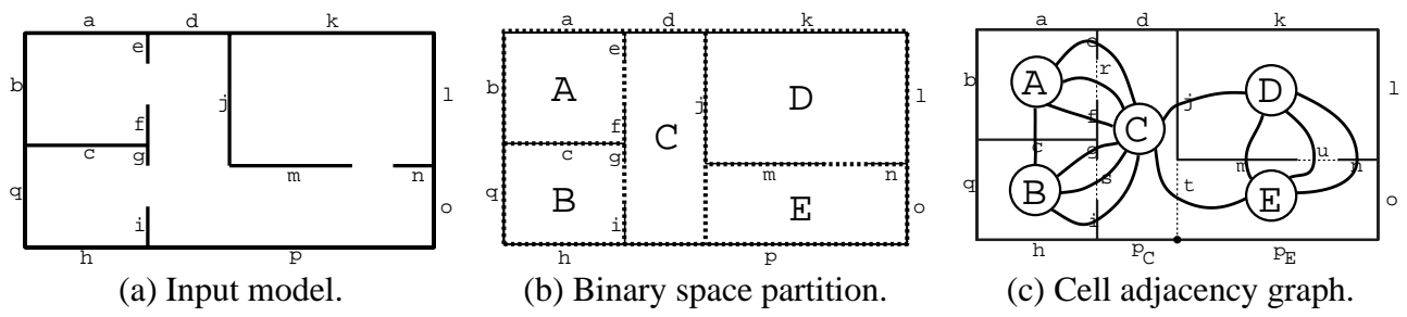
Figure 9: Example spatial subdivision.
