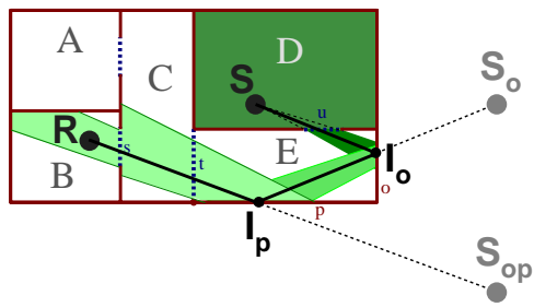
Figure 15: Propagation path to receiver point ('R') for the example in Figures 12 and 14 computed via lookup in beam tree for source point ('S').
