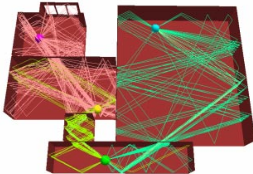
Figure 23: Sound propagation paths (lines) between four avatars (spheres) representing users in shared virtual environment.
