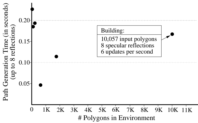
Figure 22: Path compute time vs. polygonal complexity.
