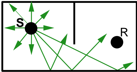
Figure 3: Ray tracing method.
