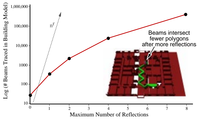
Figure 21: Plot of beam tree size with increasing reflection orders.
