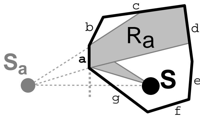
Figure 5: Beam tracing culls invisible virtual sources.
