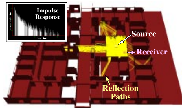
Figure 26: Impulse response (inset) derived from eighth-order specular reflection paths (yellow) in Floor model.
