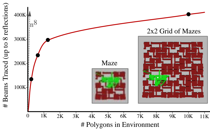
Figure 20: Plot of beam tree size vs. polygonal complexity.
