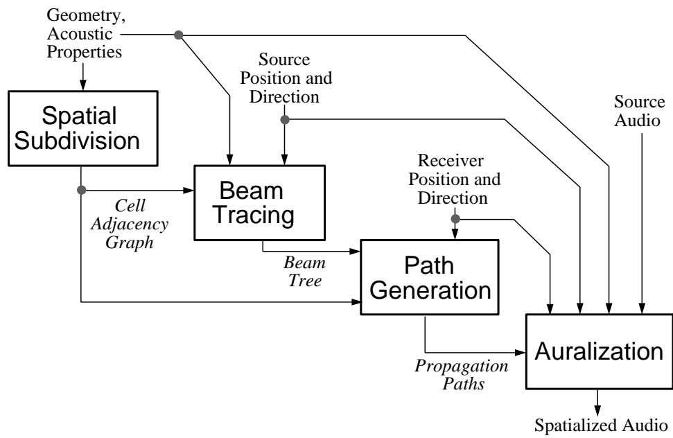
Figure 6: System organization.
