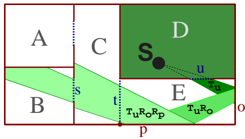
Figure 12: Beam tracing through cell adjacency graph.
