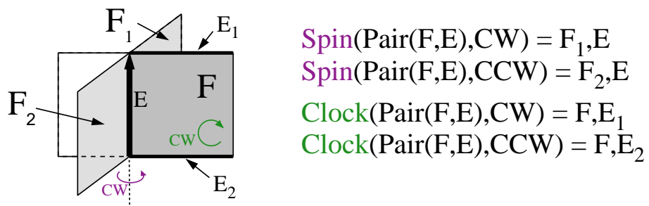
Figure 8: Winged-pair structure.
