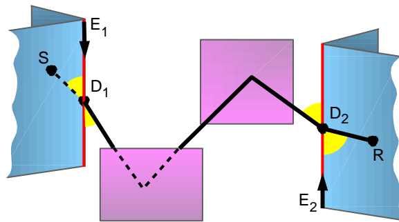
Figure 16: A single propagation path comprising a diffraction, two specular reflections, and another diffraction. The two diffraction points ( D_i ) are determined by equal angle constraints at the corresponding edges ( E_i ).
