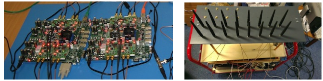
Figure 9: Left: the SecureArray prototype AP is composed of two WARP radios, while a cable-connected USRP2 software-defined radio (not shown) calibrates the array. Right: The AP and antenna array mounted on a cart.
