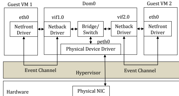
Figure 1: Xen Networking. For each guest VM, a pair of connected virtual Ethernet interfaces is created. They communicate with the help of hypervisor.
