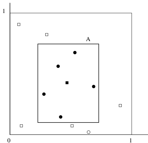
Figure 3: The rectangle A maximizes the bichromatic discrepancy for the point set shown (circles are mapped to +1 , and squares are mapped to -1 , the filled points are the ones in the interior).
