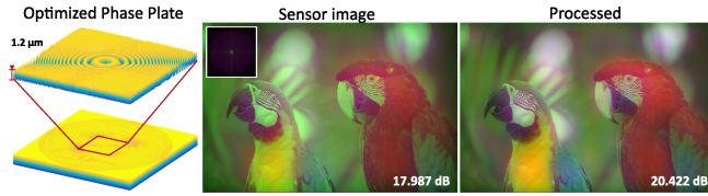
Fig. 4. Optimizing a simple optical element. We optimize a lens to focus an image at a distance of z = 25 mm without image reconstruction for a wavelength of \lambda = 550 nm. As expected, the optimized height profile (left) converges to a structure that looks similar to a Fresnel lens. As seen in the point spread function (PSF, center inset), the element is capable of focusing the green channel but residual blur remains in the other color channels because a single optical element cannot be achromatic. After deconvolving each color channel with their respective PSF, we obtain the result shown (right).
