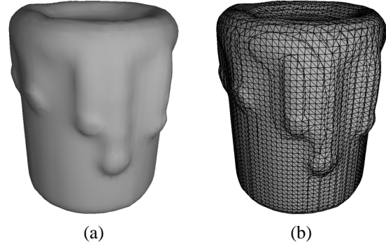
Figure 5. (a) A melting candle created with a prototype system of our modeling interface using a level set representation with a volume grid of 100x100x200 voxels. (b) The lack of adaptive resolution in the level set model prohibits the user from editing the model at various levels of detail. Moreover, this simple model took approximately 45 minutes to create due, in part, to the slow simulation speeds permitted by level sets.
